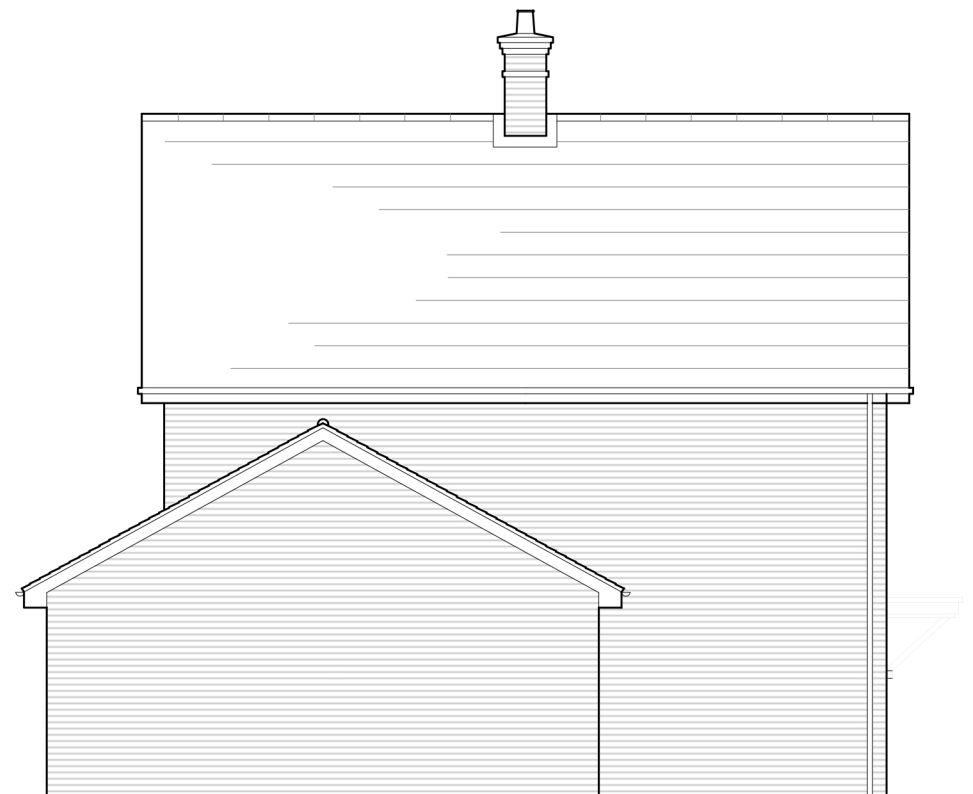
SIDE ELEVATION 2
