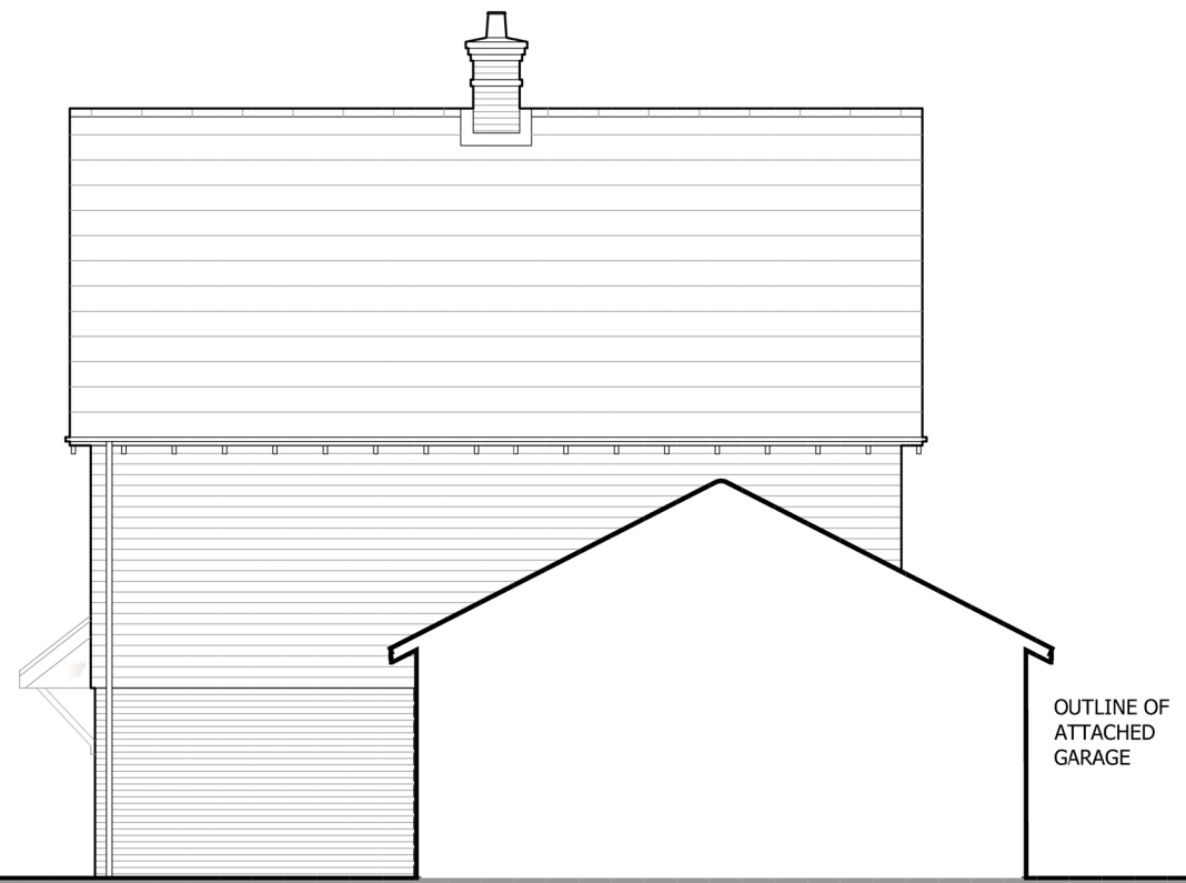
SIDE ELEVATION 1
