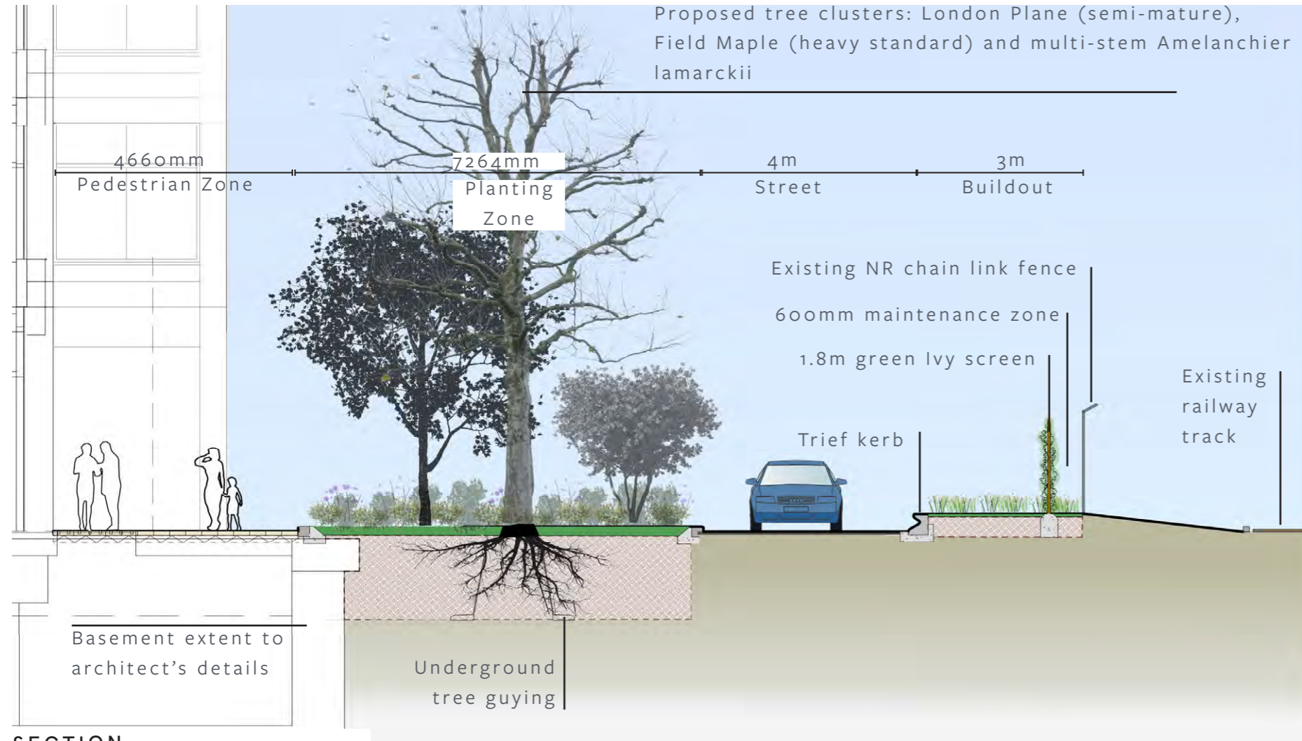
SECTION
